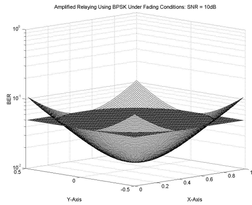
Fig. 7. Error Robustness of Amplified Relaying Multihop Channel
