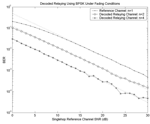
Fig. 2. Error for Decoded Reference Relaying Multihop Channel
