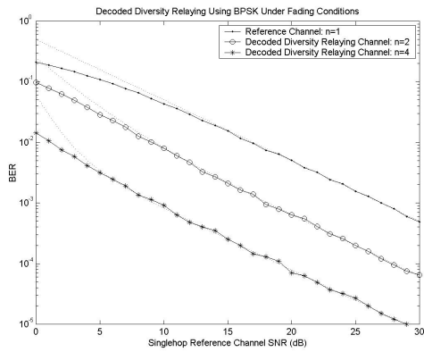
Fig. 4. Error for Decoded Relaying Multihop Diversity Channel
