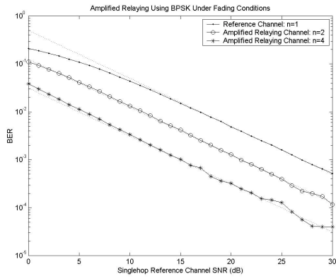
Fig. 3. Error for Amplified Relaying Multihop Channel
