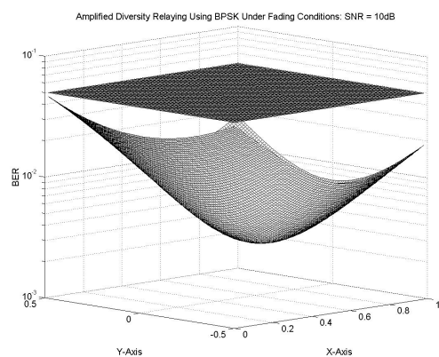
Fig. 9. Error Robustness of Amplified Relaying Multihop Diversity Channel
