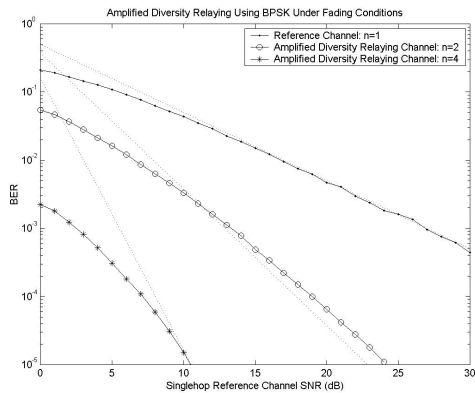
Fig. 5. Error for Amplified Relaying Multihop Diversity Channel
